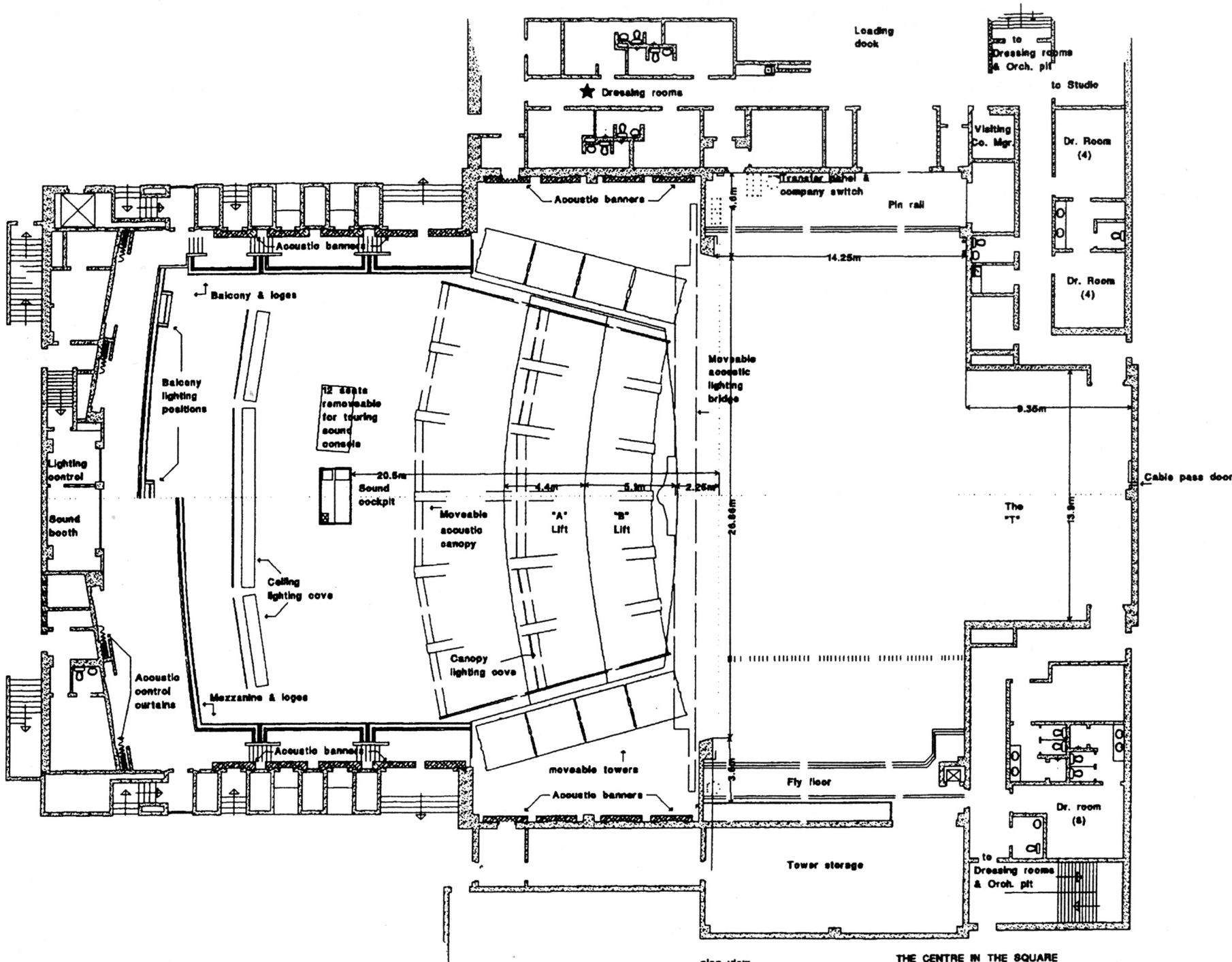
plan view
